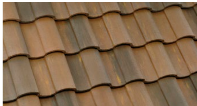
3604 Carlsbad Blend - Blend of Terracotta, Brown, Yellow Streaking Ref: .18 Emi: .88 SRI: 15 A.SRI: 16 CRRC: 0918-0055
